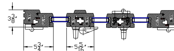
INSWING - PLAN VIEW
