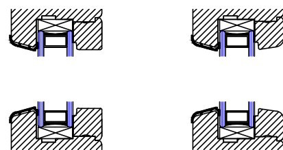
② STANDARD - SHARP & CLASSIC - SLOPED 6" = 1'-0"
