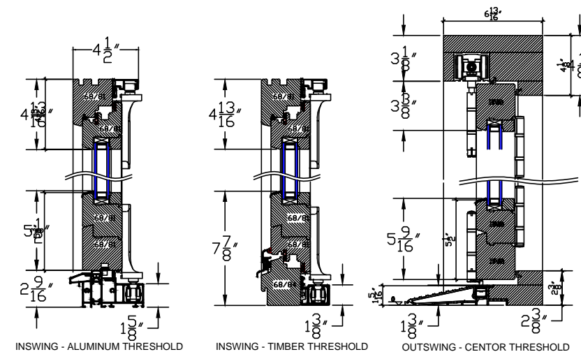
INSWING - ALUMINUM THRESHOLD INSWING - TIMBER THRESHOLD OUTSWING - CENTOR THRESHOLD
