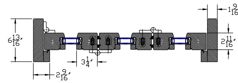
OUTSWING - PLAN VIEW
