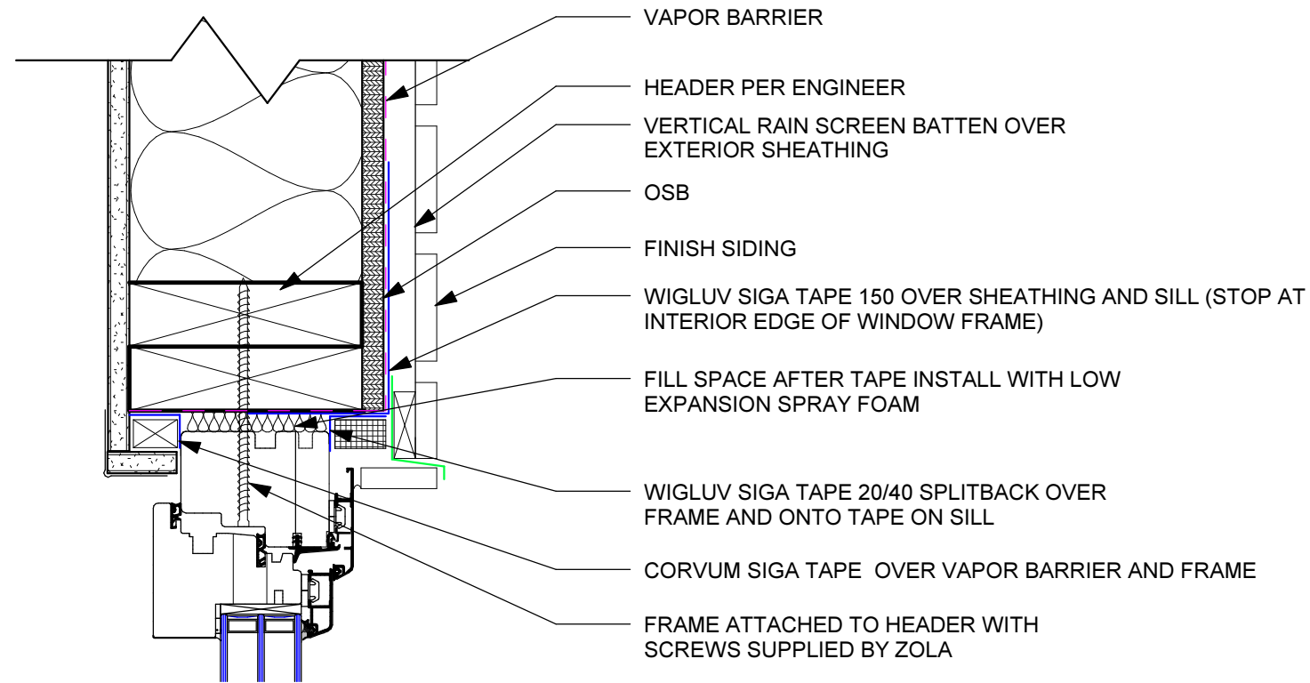
A.115 TYPICAL INSTALL DETAIL, THERMO PLUS CLAD, OPERABLE WINDOW, HEAD DETAIL 01 SCALE: 3" = 1' - 0"
