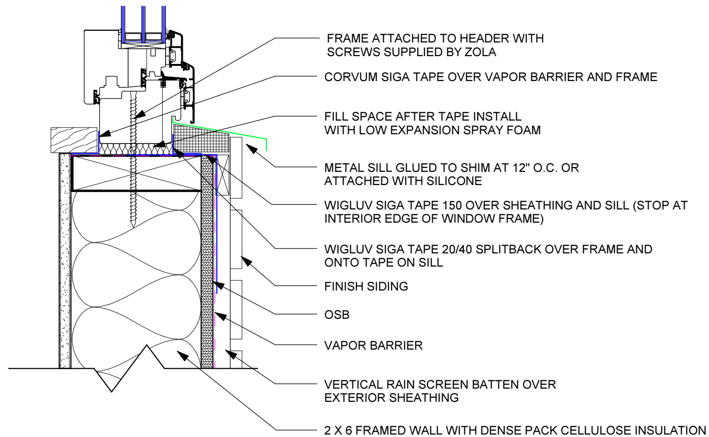
A.115 TYPICAL INSTALL DETAIL, THERMO PLUS CLAD, OPERABLE WINDOW, SILL DETAIL 02 SCALE: 3" = 1' - 0"
