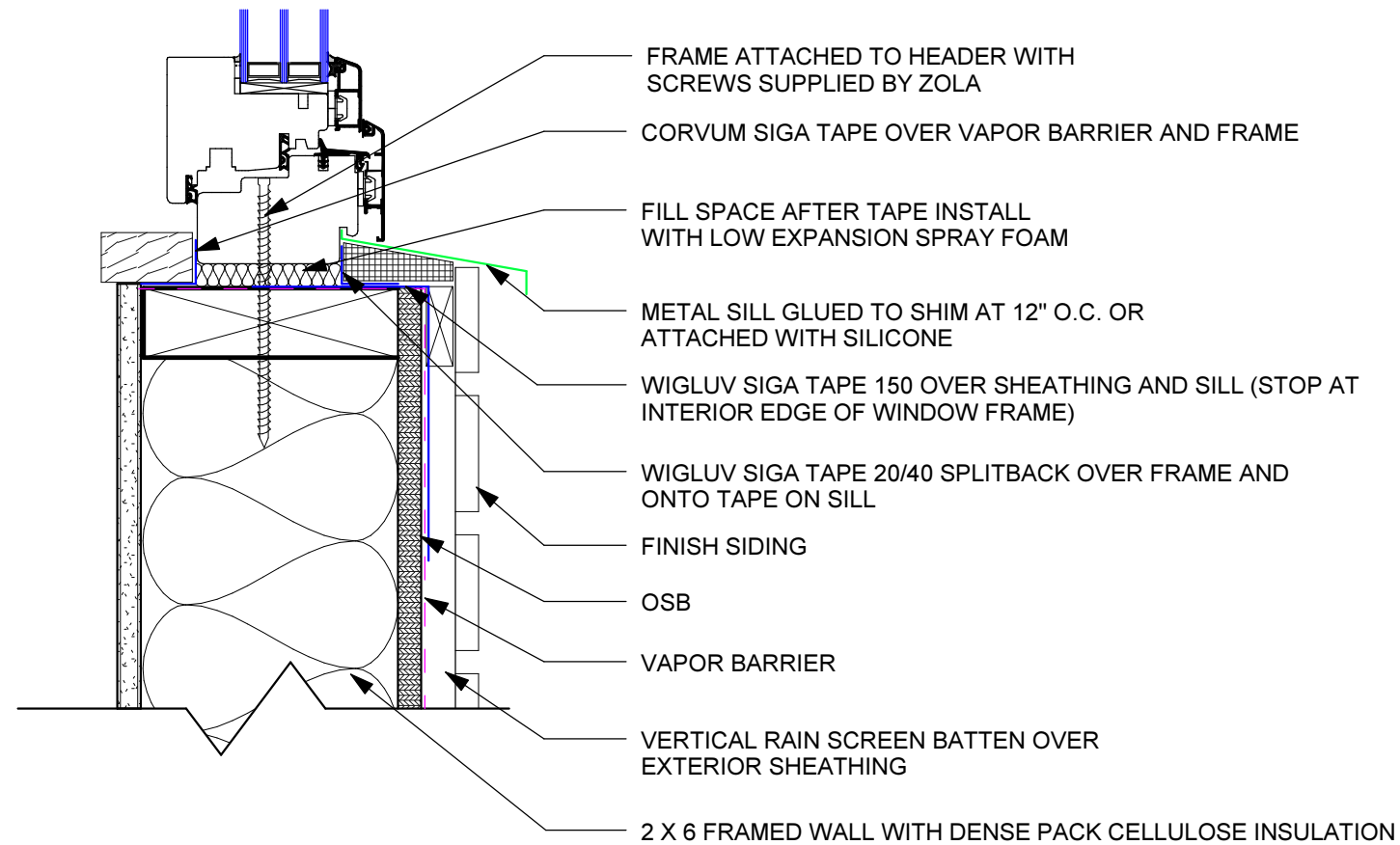
A.104 02 TYPICAL INSTALL DETAIL, THERMO CLAD, OPERABLE WINDOW, SILL DETAIL SCALE: 3" = 1' - 0"
