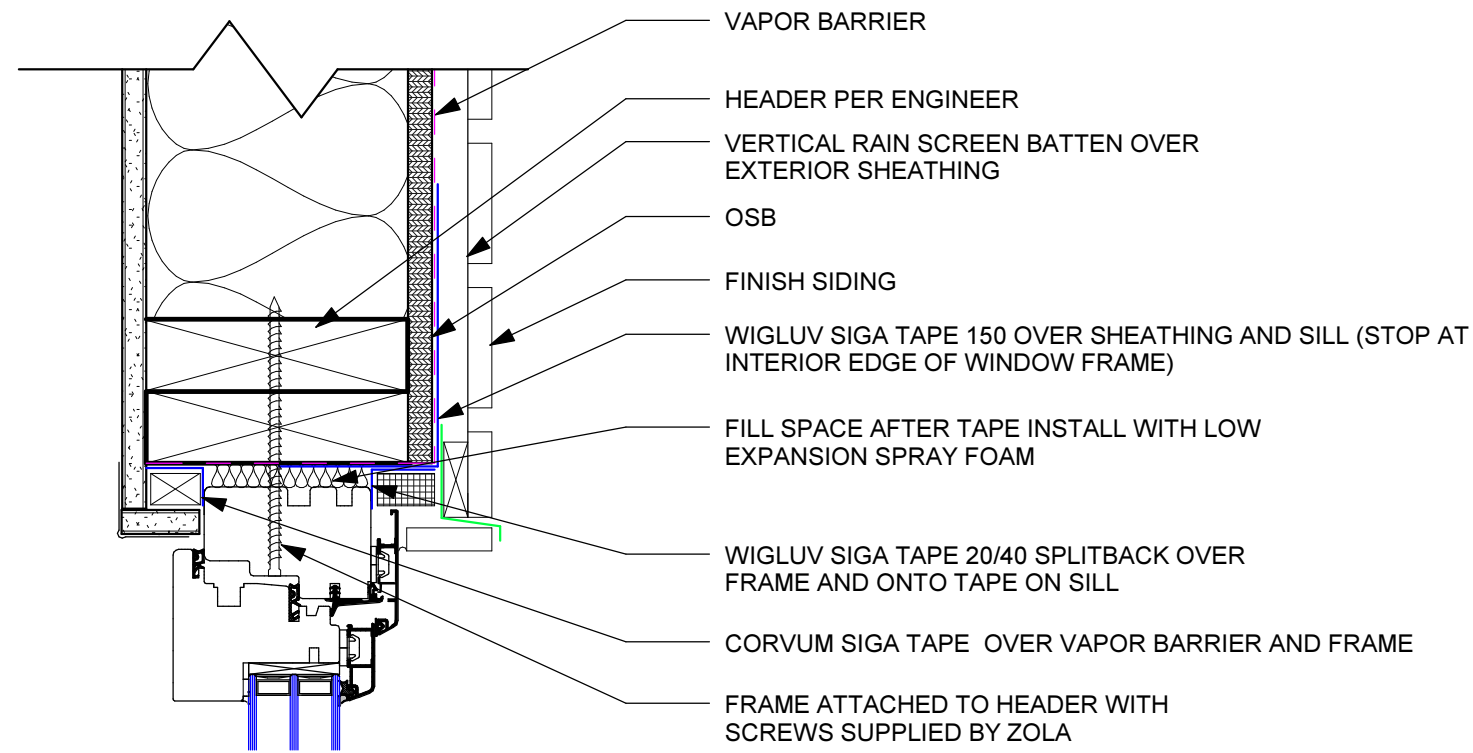
A.104 01 TYPICAL INSTALL DETAIL, THERMO CLAD, OPERABLE WINDOW, HEAD DETAIL SCALE: 3" = 1' - 0"
