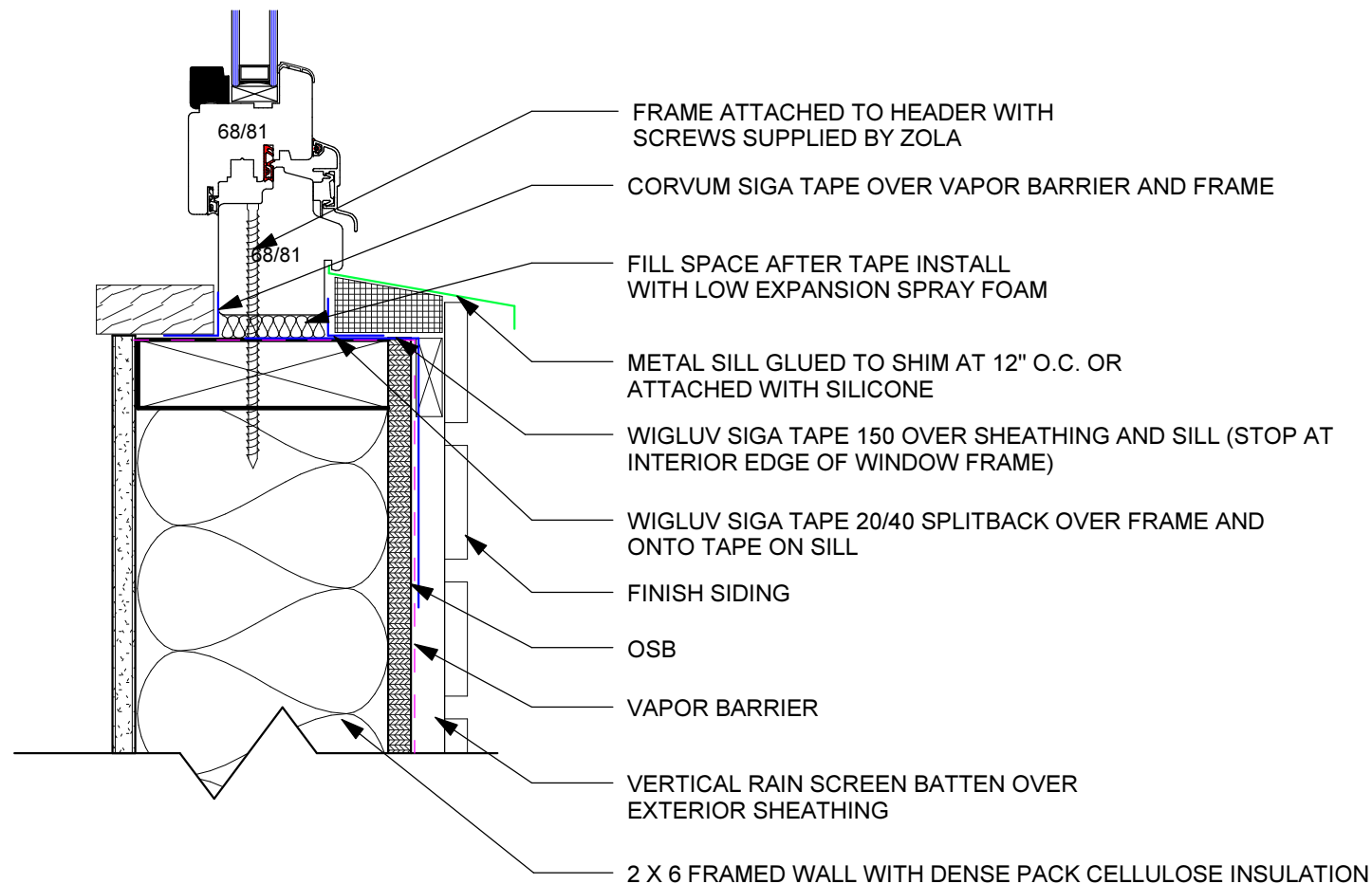
A.114 02 TYPICAL INSTALL DETAIL, CLASSIC WOOD, OPERABLE WINDOW, SILL DETAIL SCALE: 3" = 1' - 0"
