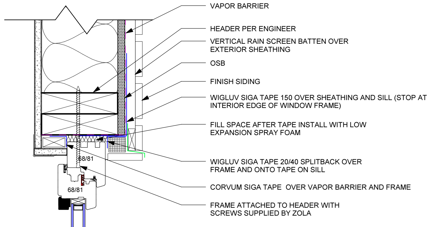
A.114 01 TYPICAL INSTALL DETAIL, CLASSIC WOOD, OPERABLE WINDOW, HEAD DETAIL SCALE: 3" = 1' - 0"
