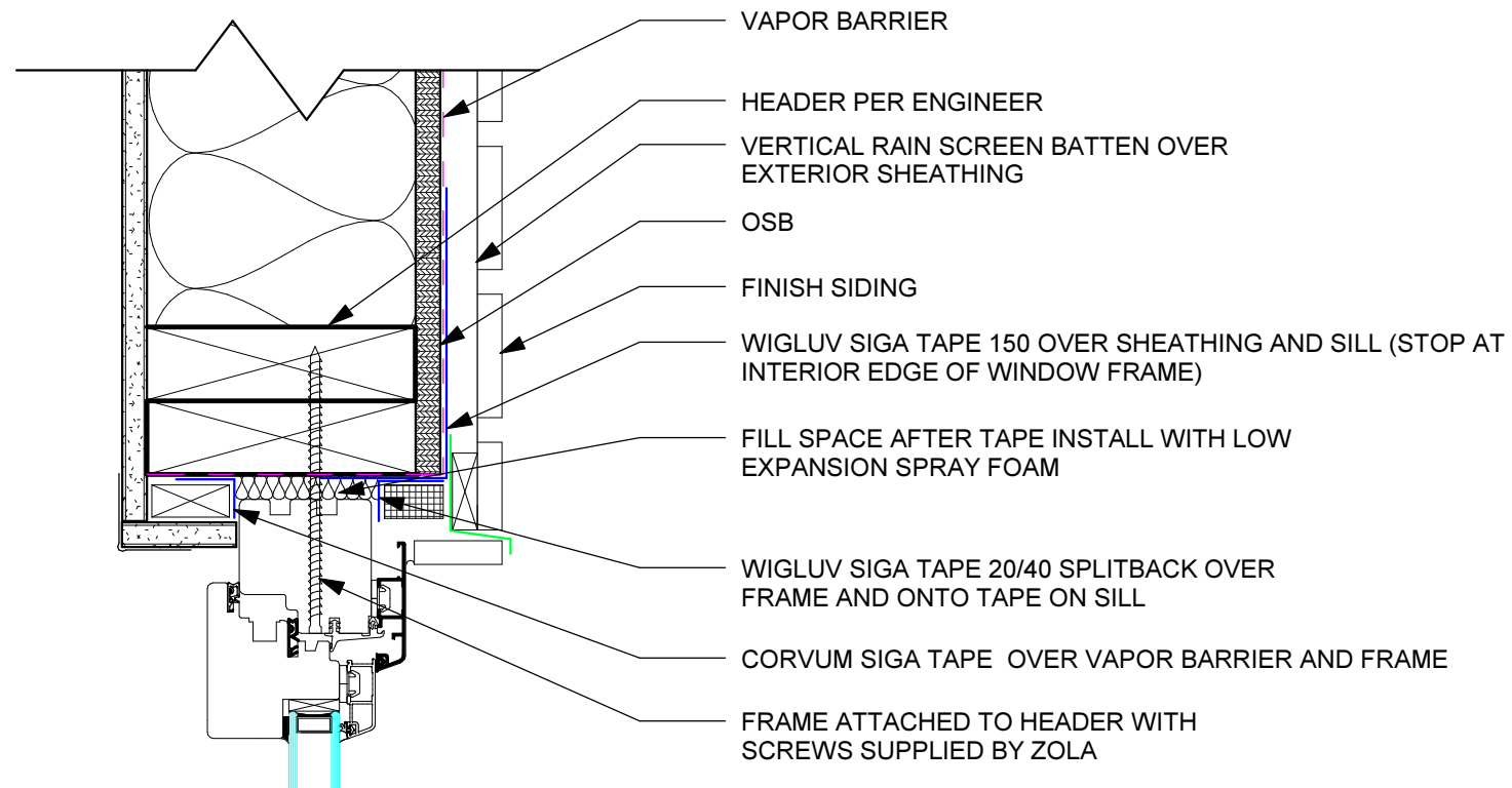
A.113 01 TYPICAL INSTALL DETAIL, CLASSIC CLAD, OPERABLE WINDOW, HEAD DETAIL SCALE: 3" = 1'-0"
